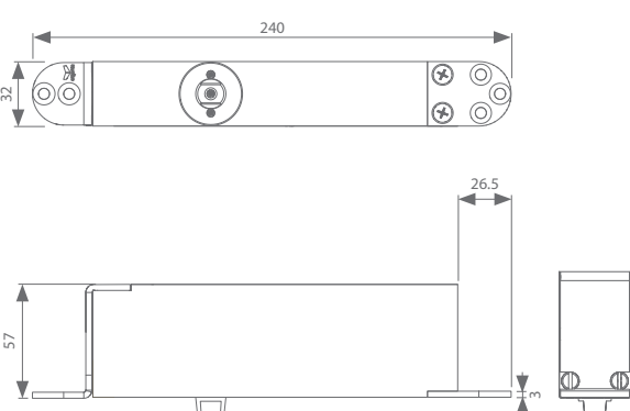
Bottom part door - centre or off-centre position
