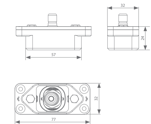
Bottom part door - centre or off-centre position
