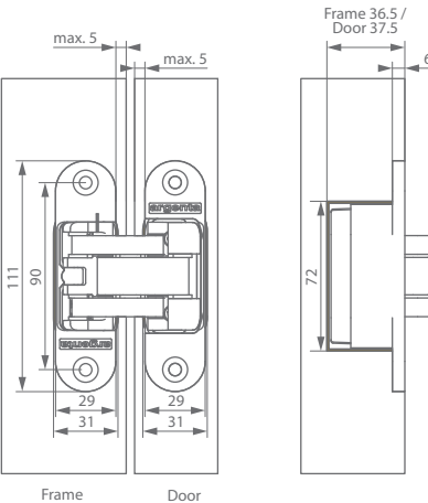
invisible medium fire resistant
