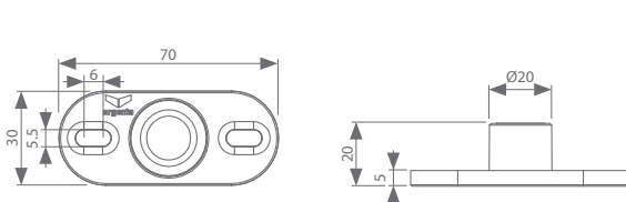
Top part of door opening
