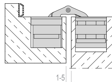
Section of Wood Frame-Door Installation
