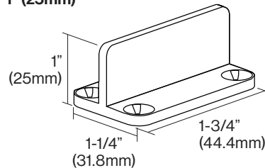
Standard T-Guide 1" (25mm)
