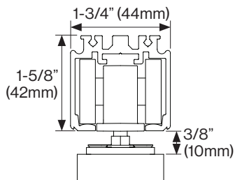
Minimum Clearance
