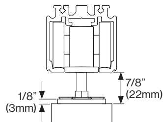
Maximum Clearance
